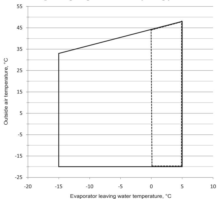
Operating range with 45% ethylene glycol
