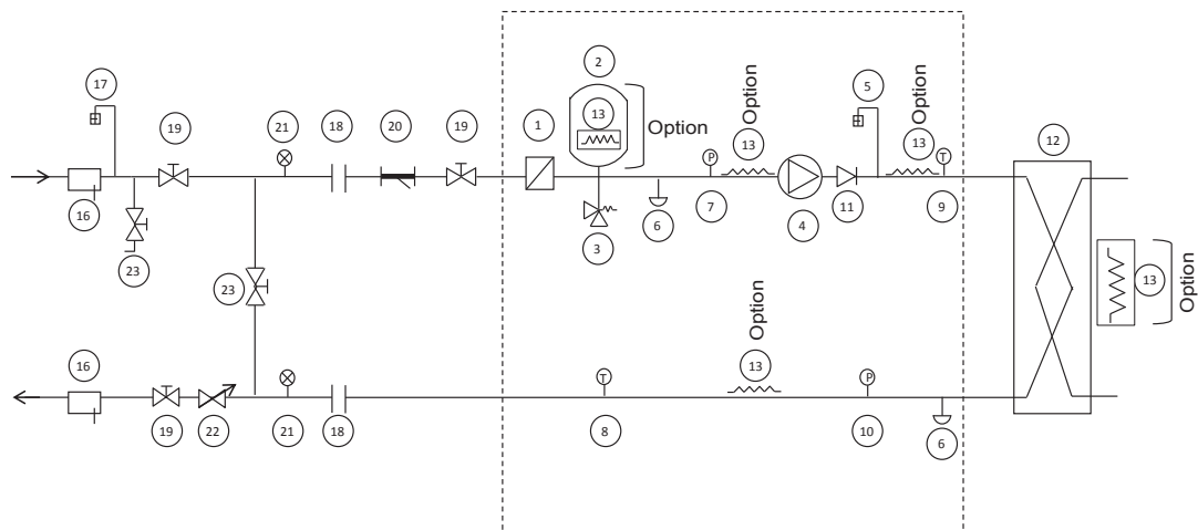
Typical hydraulic circuit diagram
