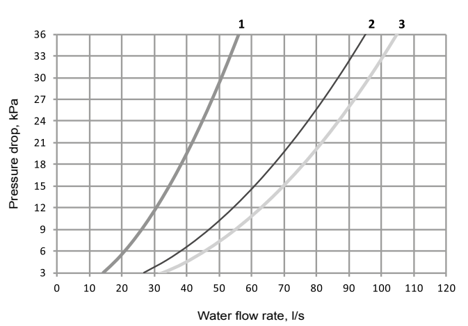
Units with one evaporator pass (option 100C)
